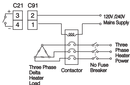
Figure 2.15 Output 2 Relay or Triac (SSR) to Drive Contactor
