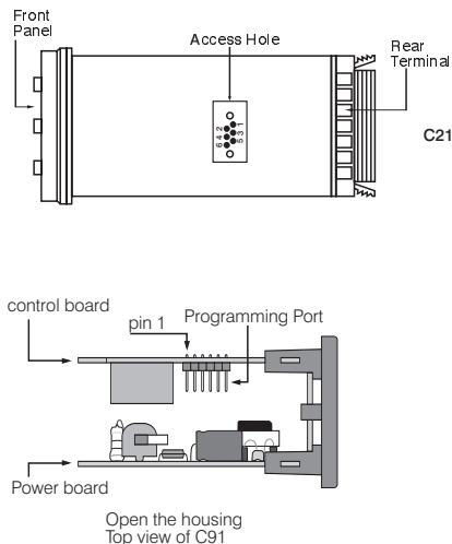
Figure 1.2 Programming Port Overview
