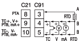
Figure 2.8 Sensor Input Wiring
