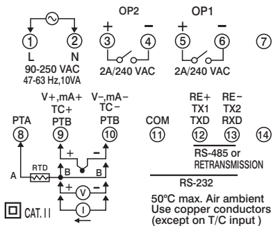
Figure 2.4 Rear Terminal Connection for C21
