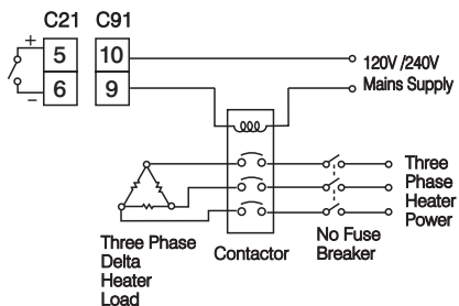
Figure 2.10 Output 1 Relay or Triac (SSR) to Drive Contactor
