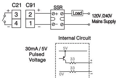
Figure 2.16 Output 2 Pulsed Voltage to Drive SSR
