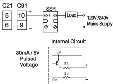
Figure 2.11 Output 1 Pulsed Voltage to Drive SSR
