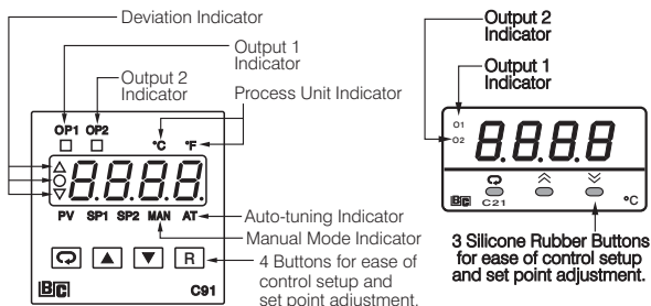
Figure 1.3 Front Panel Description
