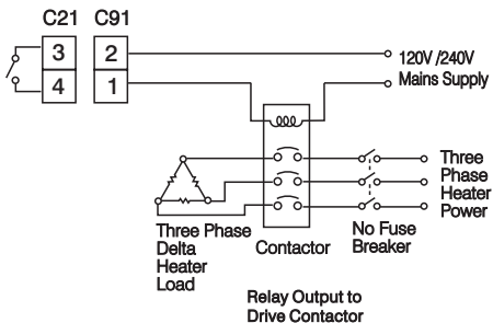
Figure 2.20 Alarm Output to Drive Contactor
