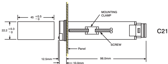
Figure 2.1 Mounting Dimensions
