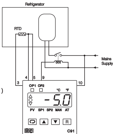
Figure 4.2 Cooling Control Example
