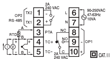
Figure 2.5 Rear Terminal Connection for C91
