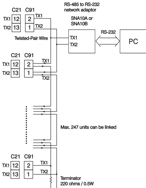
Figure 2.21 RS-485 Wiring
